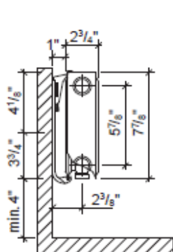
RCV21S Baseboard
