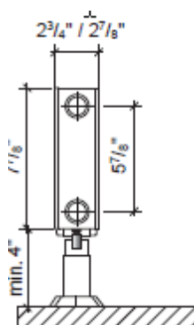
CV21S Pedestal
