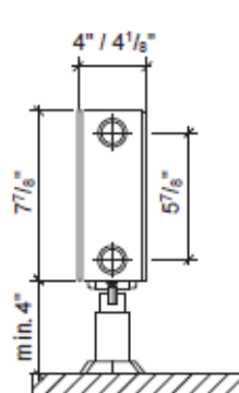
RCV22 Pedestal
