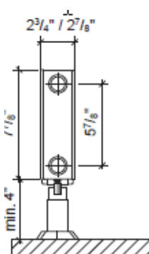
RCV21S Pedestal
