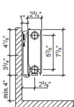
CV21S Baseboard
