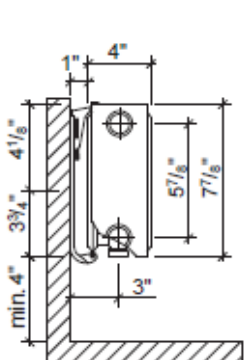
RCV22 Baseboard
