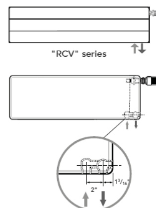
RCV22 Pedestal
