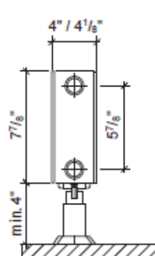
CV22 Pedestal
