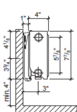
CV22 Baseboard
